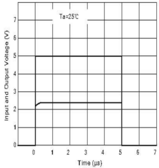
Fig 4 Pulse Response
