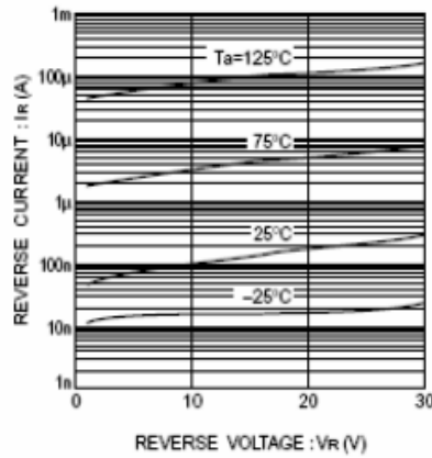
Fig. 2 Reverse characteristics
