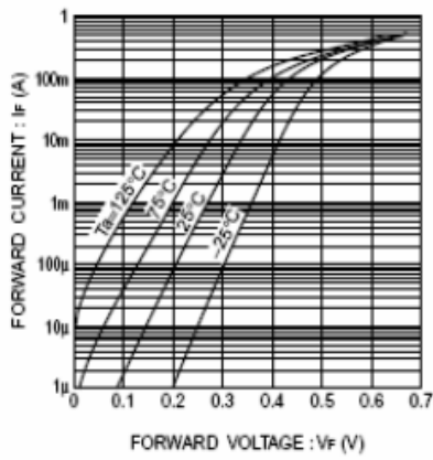
Fig. 1 Forward characteristics
